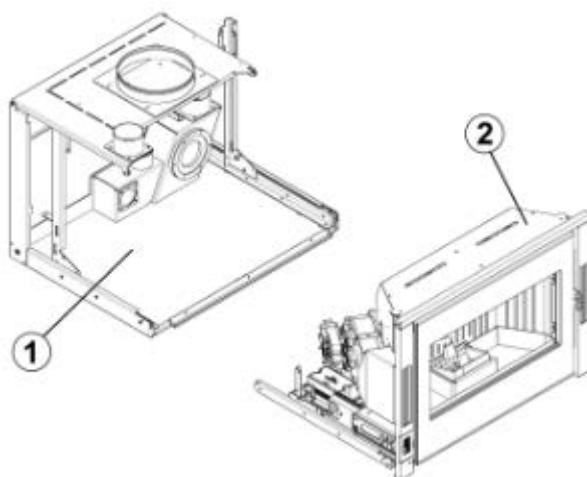
Fig. 25 - Structure + corps machine
